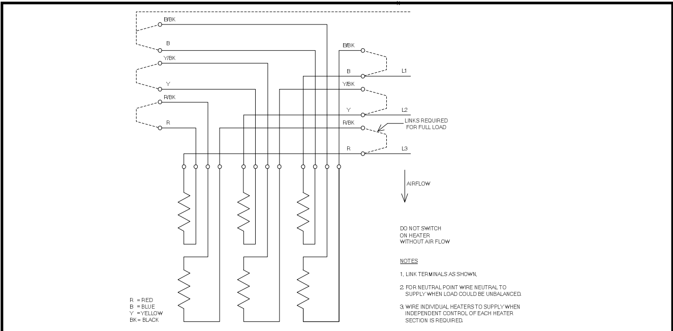
WIRING DETAILS
